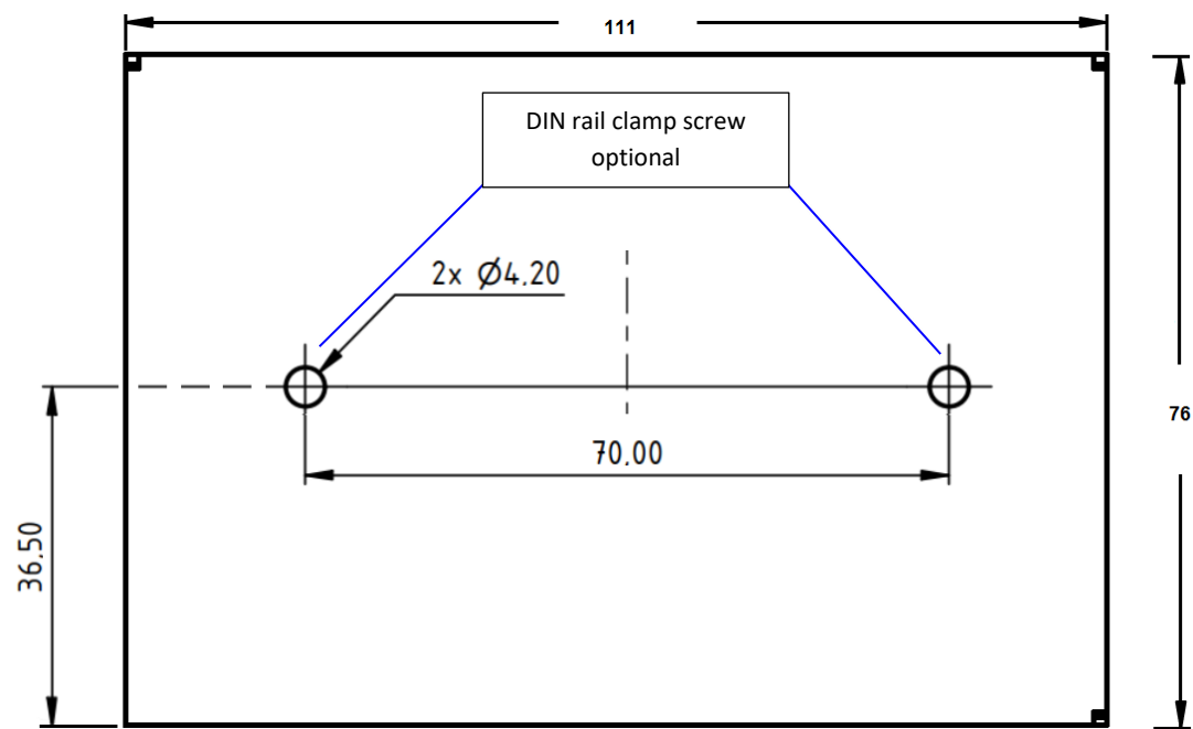
Figure 2: Bottom view
